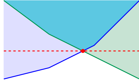
(b) Linear programming formulation.
