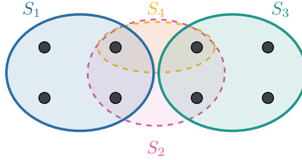
Figure 8.1: A set cover instance: a universe U of elements (dots) and four weighted sets S_1, \dots, S_4 (ellipses); the goal is a minimum-weight sub-collection of sets that covers every element of U .
