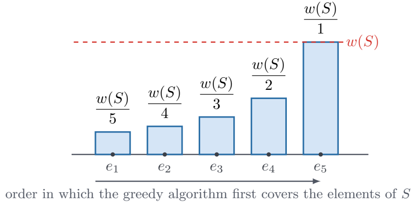
Figure 8.2: Dual fitting, viewed through one set S = \{e_1, \dots, e_k\} with its elements ordered as the greedy algorithm first covers them. When e_i is covered at least k - i + 1 elements of S remain, so its dual charge is y'_{e_i} \leq w(S)/(k - i + 1) ; the charges grow harmonically and sum to at most w(S) H_k \leq w(S)(\ln k + 1) , which is why scaling y' down by \ln n + 1 yields a feasible dual.
